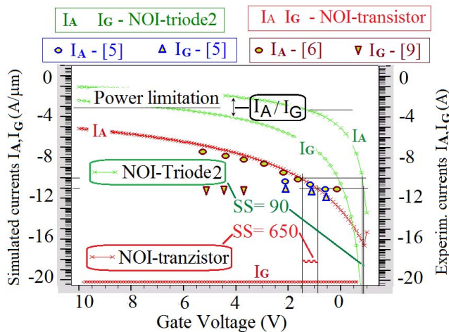
FIGURE 9. Comparative curves I_A - V_G and I_G - V_G at V_A = 0.6V for the NOI-transistor with SS = 650mV/dec and NOI-triode2 with SS = 90mV/dec ; experimental picked points are measured at V_A = 1V for [5], [6].
